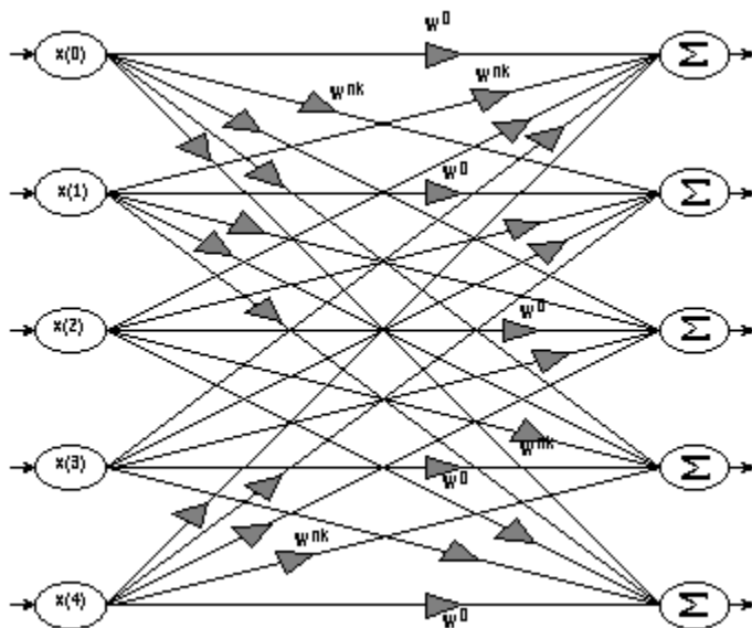
Figure 2.2 Flow diagram for a radix 5 butterfly.
