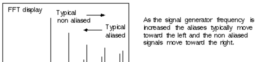
Figure 1.19 Change the generator frequency to identify aliases.
