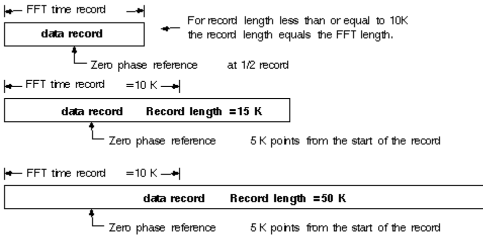
Figure 1.1 Relationship of the FFT time record to the acquired data record.
