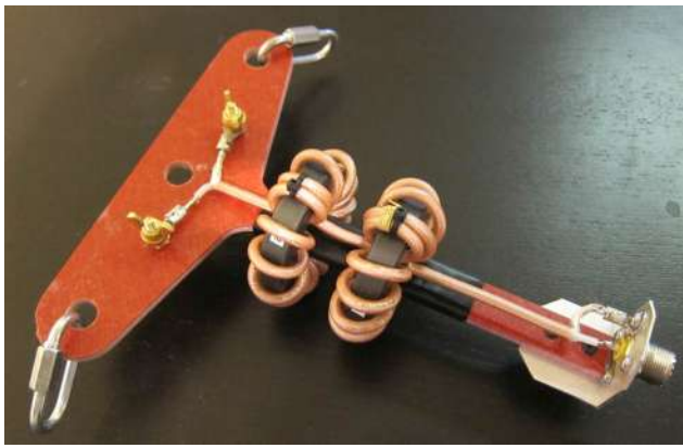
Fig 11 – W6GJB's Dipole Center Insulator With Two RG400 Chokes
