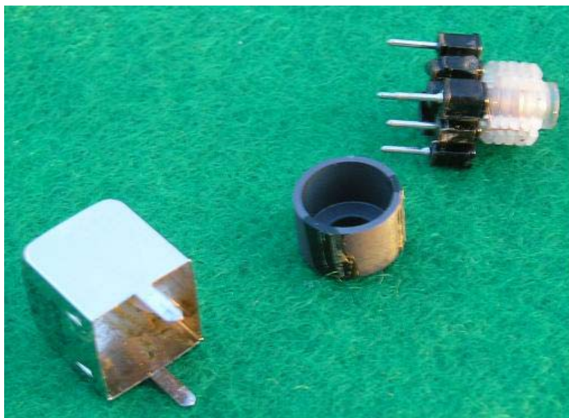
Fig 2 – the 10K Components – can, cup and bobbin
