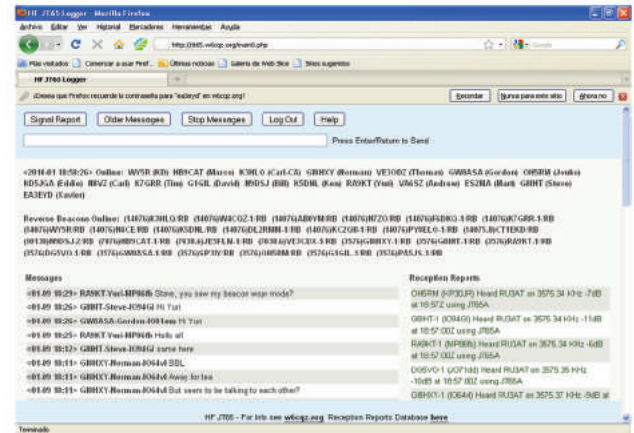
Baliza JT65A
